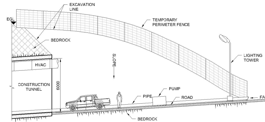
SECTION THROUGH CONSTRUCTION TUNNEL PORTAL CONSTRUCTION
