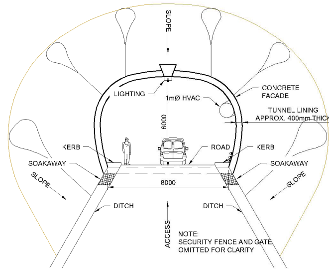
ELEVATION CONSTRUCTION TUNNEL OPERATION 1:125
