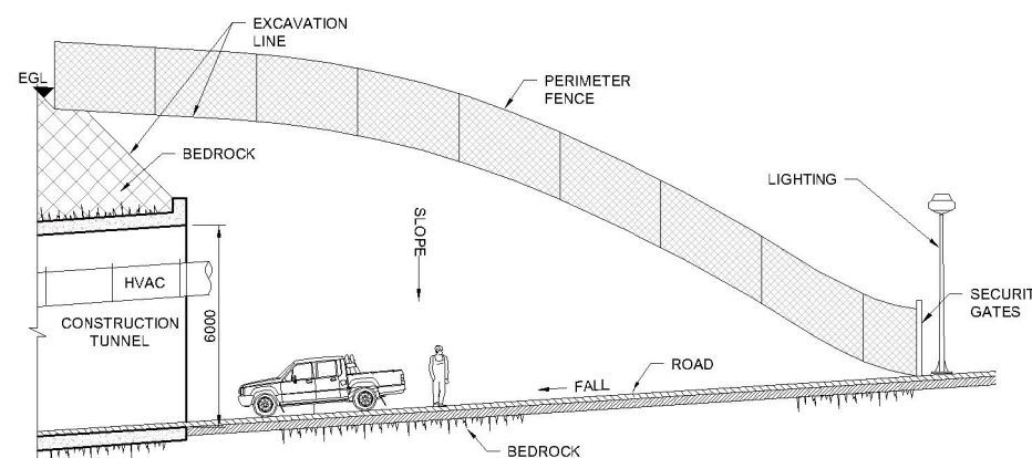
SECTION THROUGH CONSTRUCTION TUNNEL PORTAL OPERATION
