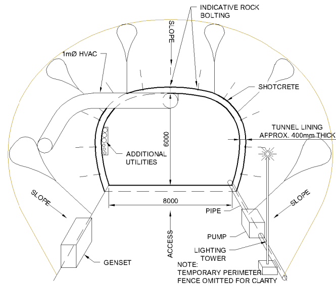
ELEVATION CONSTRUCTION TUNNEL CONSTRUCTION 1:125
